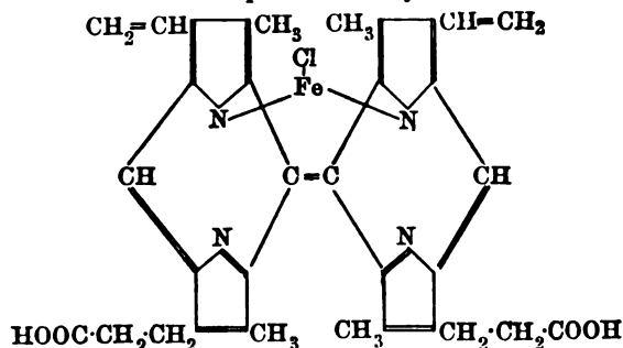
Haemin, C_{38}H_{38}N_4O_4FeCl .
